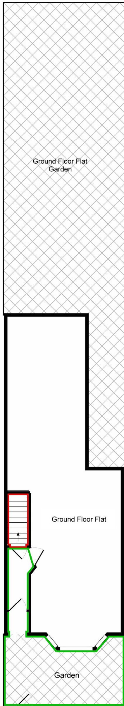
GROUND FLOOR
